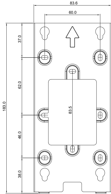
1 FRONT VIEW
