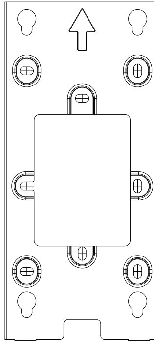
2 FRONT VIEW:WALL MOUNTING BRACKET PLACEMENT
